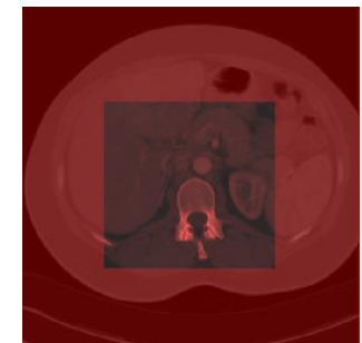
Masking
