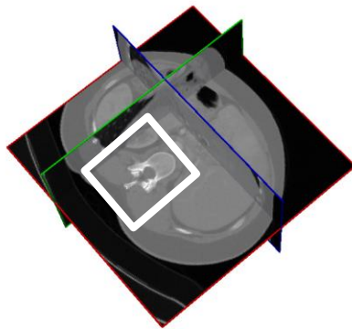
Whole volume
