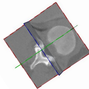
Cropped volume
